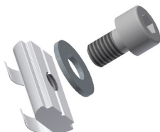
Set of 10 M5 T-slot nuts with spring for aluminium extrusion profile mounting
